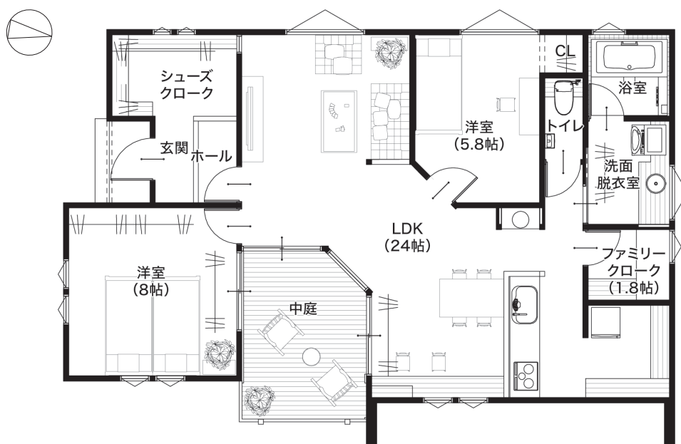
1F Plan
