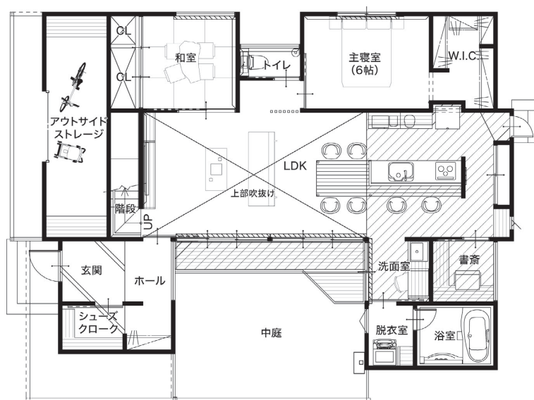
1F Plan
